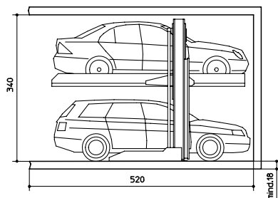
Wöhr-Parklift 411-D-165 Standard type
