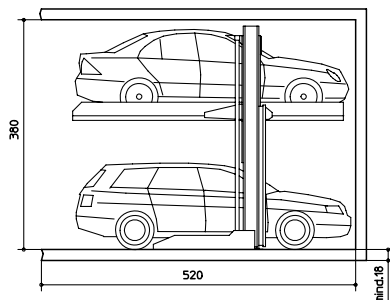
Wöhr-Parklift 411-D-205 Comfort type
