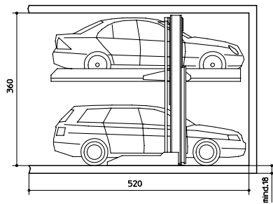
Wöhr-Parklift 411-S-195 Comfort type
