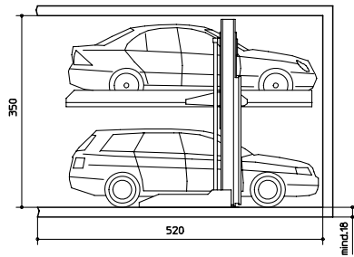
Wöhr-Parklift 411-D-175 Standard type
