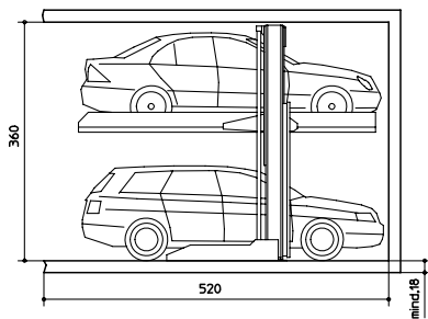
Wöhr-Parklift 411-D-185 Comfort type
