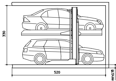
Wöhr-Parklift 411-D-155 Standard type
