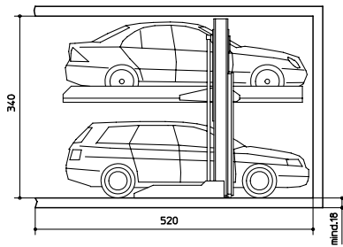
Wöhr-Parklift 411-S-175 Standard type
