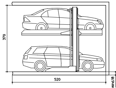
Wöhr-Parklift 411-D-195 Comfort type
