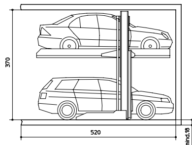
Wöhr-Parklift 411-S-205 Comfort type
